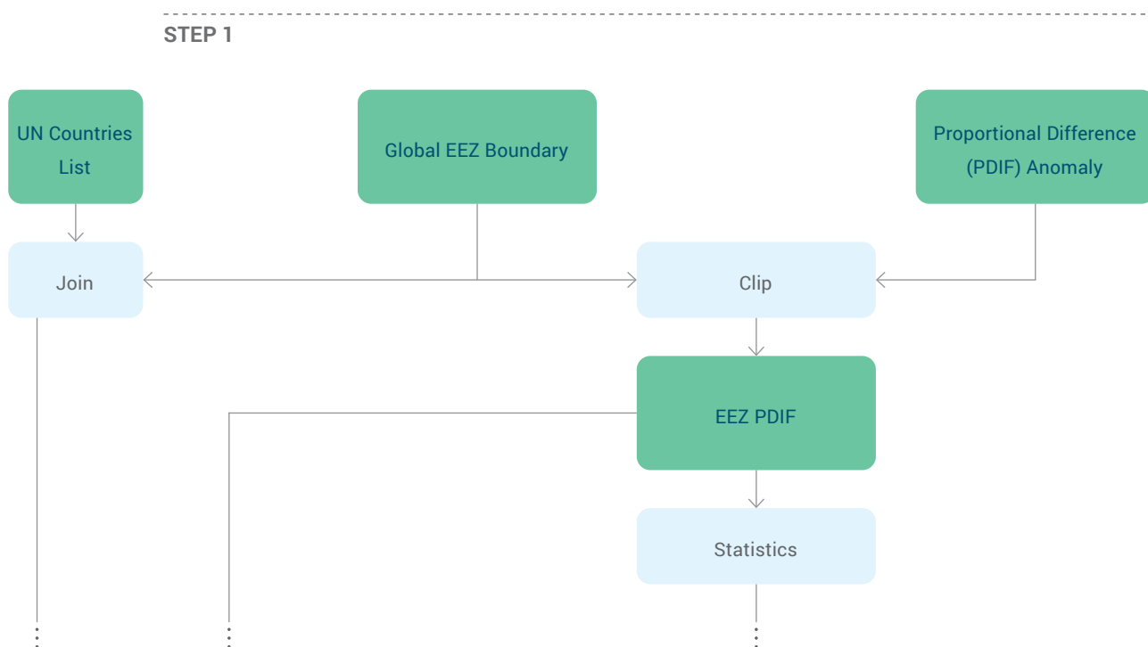
Figure 5: Process for Calculating the Intra-annual EEZ Chlorophyll-a Anomalies
